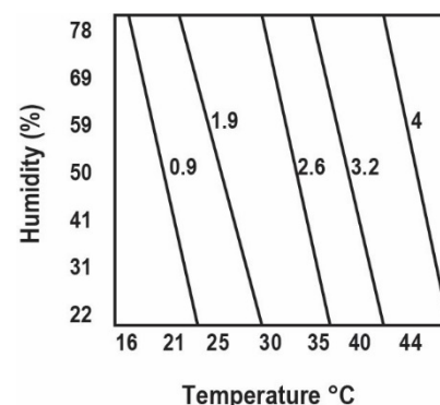
Figure 2: Cure in depth after 24 hours.
